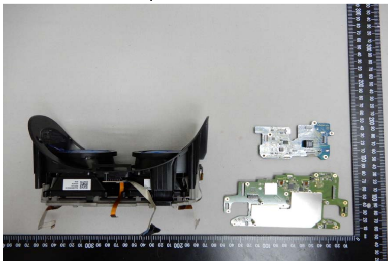
Internal View of EUT - 1
