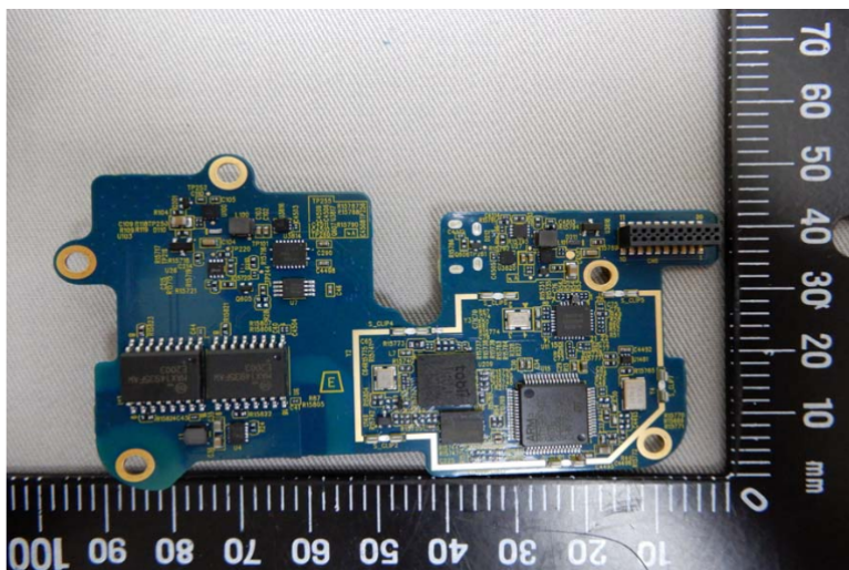
Internal View of EUT - 3
